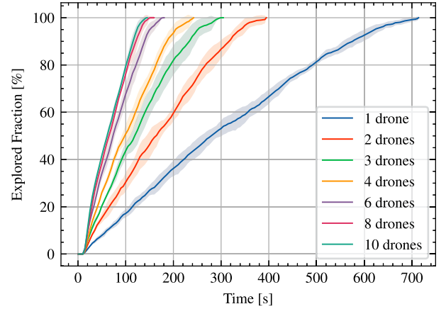
Fig. 4. Exploration rates over different numbers of UAVs in the forest with density 0.1 trees / m 2 . The exploration process becomes more efficient as the size of the fleet increases.
