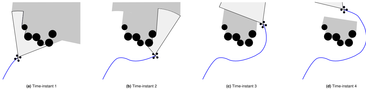
Fig. 2. Schematic example demonstrating the problem with greedy frontier-based exploration, at progressive time-instants, generating islands of unknown space surrounded by free regions. The field of view of the robot is depicted as a light-gray shaded area delimited by black solid lines, while the obstacles and the unexplored space are in black and dark gray, respectively (Fig. 2(a)). The robot navigates towards the most informative frontiers (Fig. 2(b)). However, due to the limited sensor range, the space occluded by the obstacles is not cleared (Fig. 2(c)). Consequently, since the exploration process is biased towards larger, more informative frontiers, the naive planner flies the UAV robot ignoring the smaller portion of unexplored space shown in dark gray (Fig. 2(d)).
