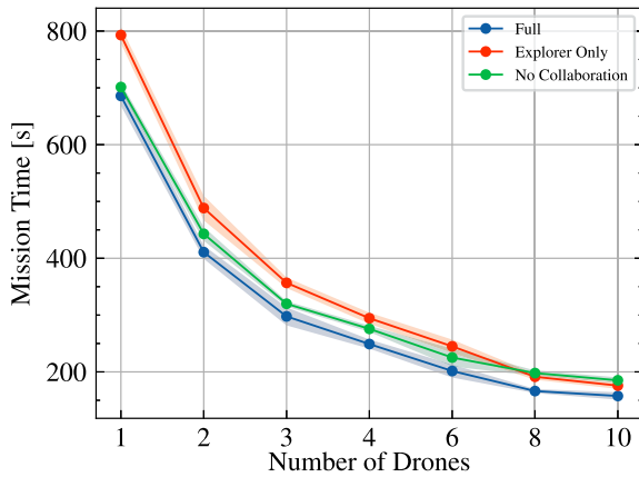
Fig. 7. Average exploration times in the reconstruction of a real forest [8] over 5 runs. The standard deviation is shown as a shaded area. We compare the proposed strategy ( Full ) against two variants, namely Explorer Only , where UAVs are not allowed to switch to Collector mode, and No Collaboration , where inter-agent coordination is ignored. The proposed pipeline shows the best performance.
