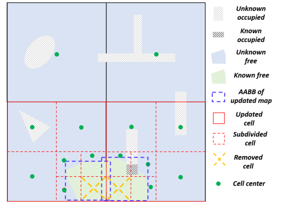
Fig. 3. Illustration of the procedure to update a three-level hgrid. Cells that overlap with any AABBs in \mathcal{B}_m are updated and subdivided into finer cells if necessary. Cells that have been covered completely are removed from \mathcal{L}_{act} .
