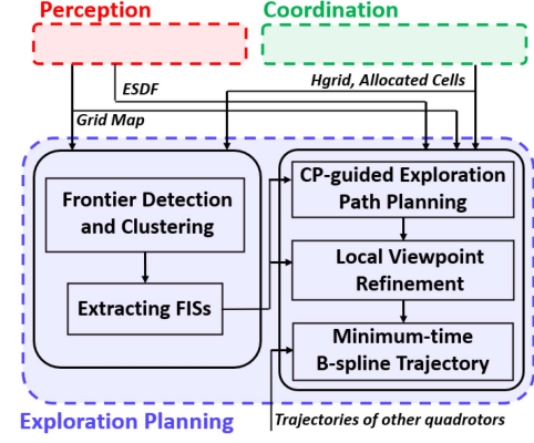
Fig. 6. Detailed components of the exploration planning module.
